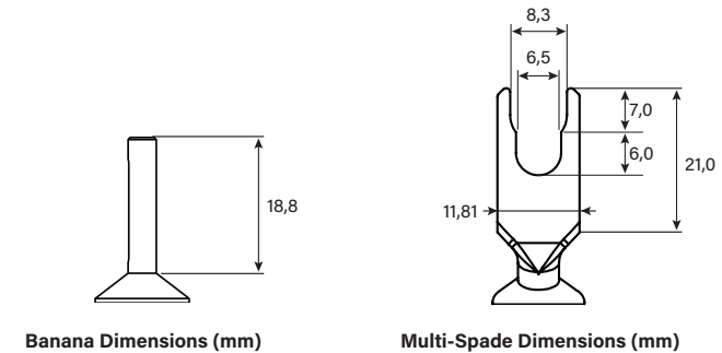
Banana Dimensions (mm)
